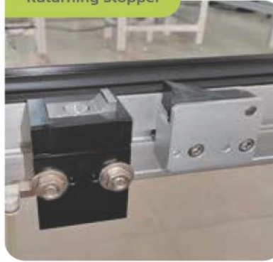
Returning Stopper
