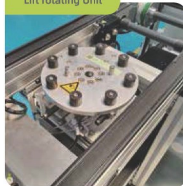
Lift rotating Unit
